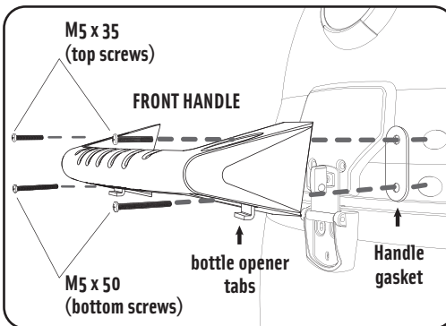
STEP 4: Attach front handle with Phillips head screwdriver. M5x50 screws go in the bottom holes with the bottle opener tabs. M5x35 screws go in the top holes. Silicone gaskets install behind handle (two places).
