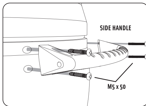
STEP 5: Attach side handles (2) using 4 (M5 x 50) screws. (Use Phillips head screwdriver)
