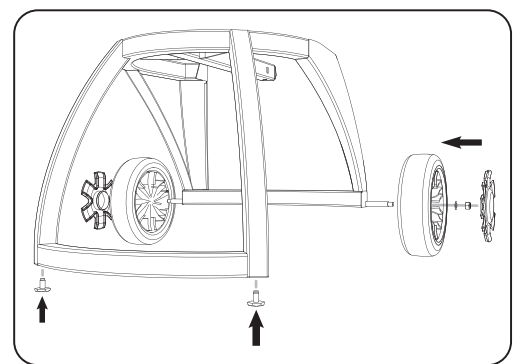
STEP 6: Attach both wheels to the axle posts on the stand in the following order: wheel, washer nut and hub cap. Use ½ inch or 13mm wrench. Then screw in leveling feet to stand.
